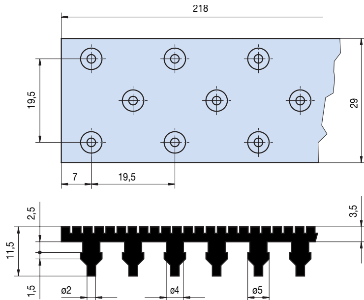
GU1 rubber jaw liner with retaining studs
