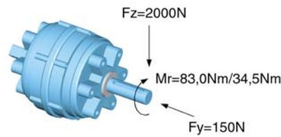
Max Allowable Forces on Jaws
