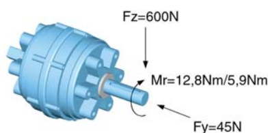
Max Allowable Forces on Jaws
