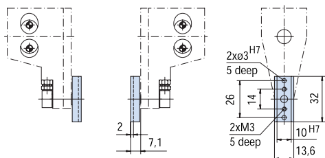
Slotted jaw Order no.: SB32-1
