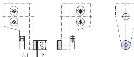
Rubber Jaws Order no.: SB32-2
